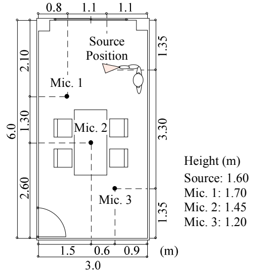
Figure 11: Schematic diagram of the arrangement used to measure reverberation time.
